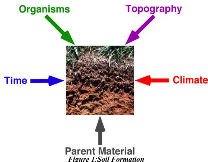
Figure 1: Soil Formation
