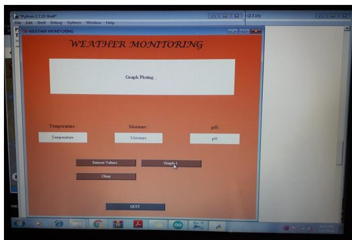
Figure 5:GUI
